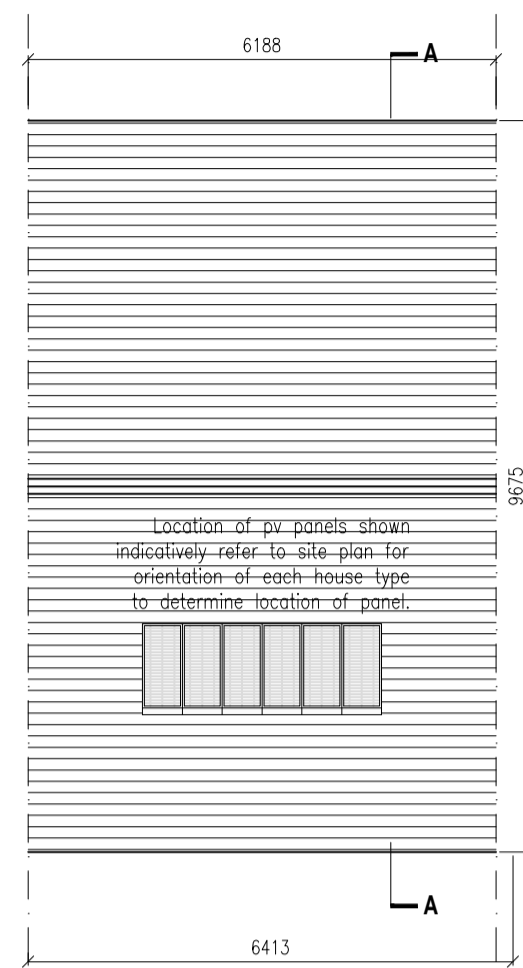
Roof Plan
