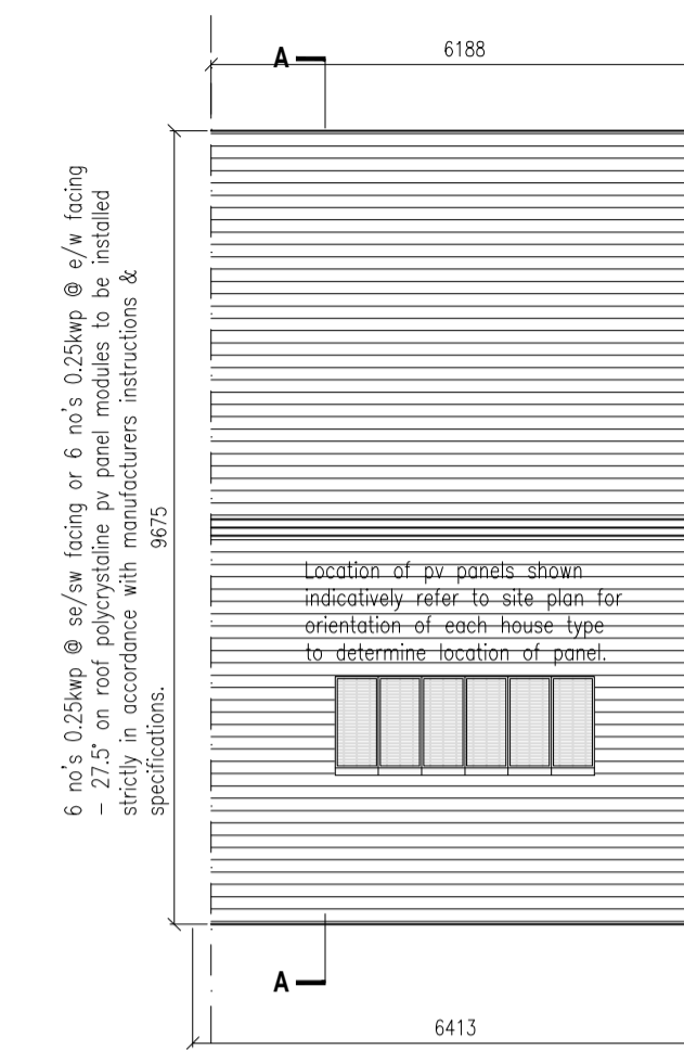
Roof Plan
